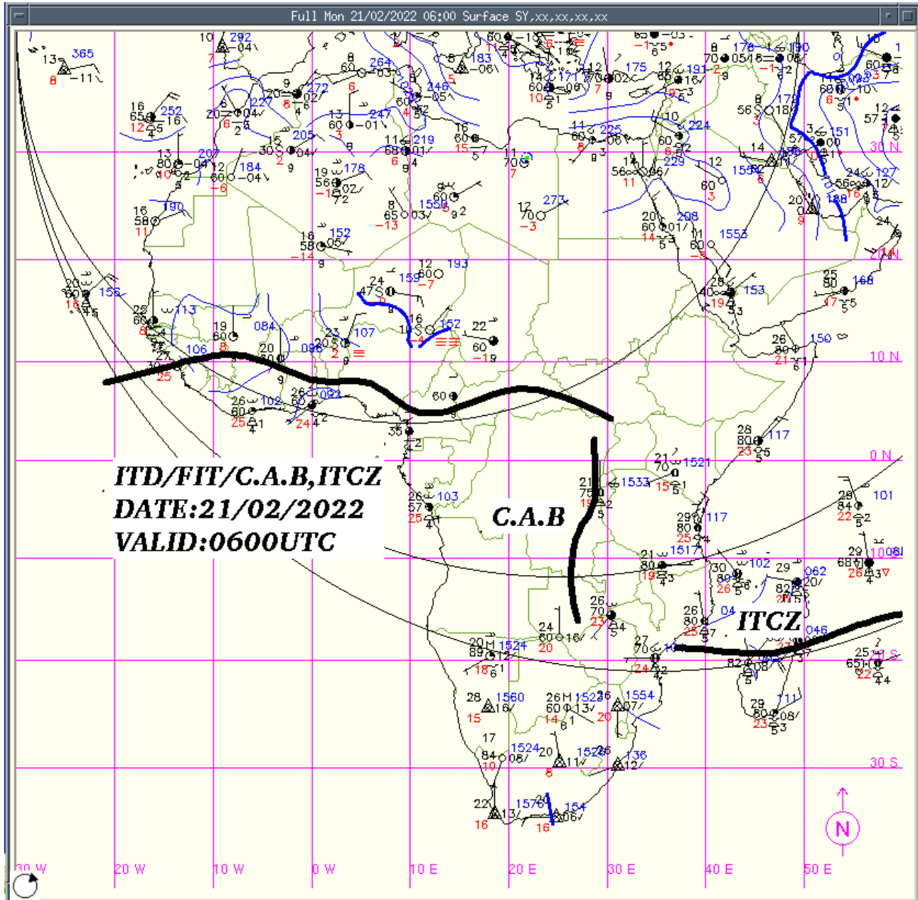
Tabulated positions of the ITD: 21 st February 2022
