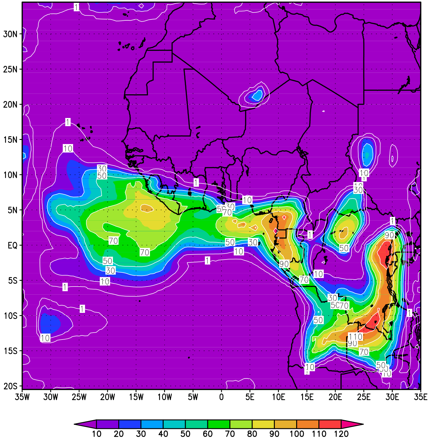
ACMAD GISS RM3 24h rainfall; valid T+72H; from 00Z on Mon Nov 2 2015
