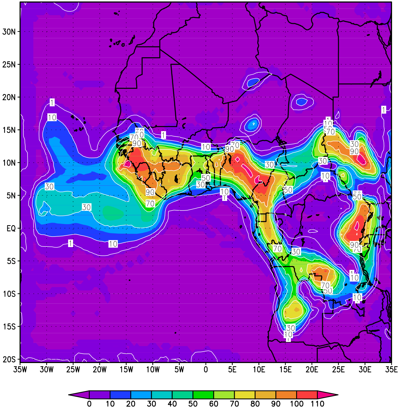
ACMAD GISS RM3 24h rainfall; valid T+72H; from 00Z on Thu Aug 4 2016
