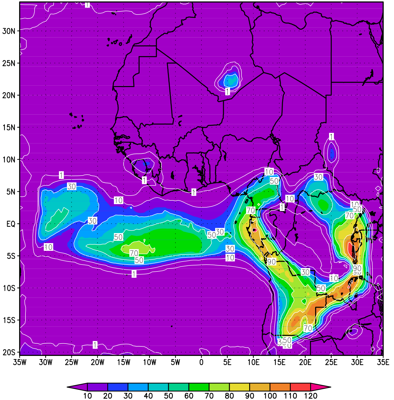
ACMAD GISS RM3 24h rainfall; valid T+72H; from 00Z on Sat Dec 5 2015
