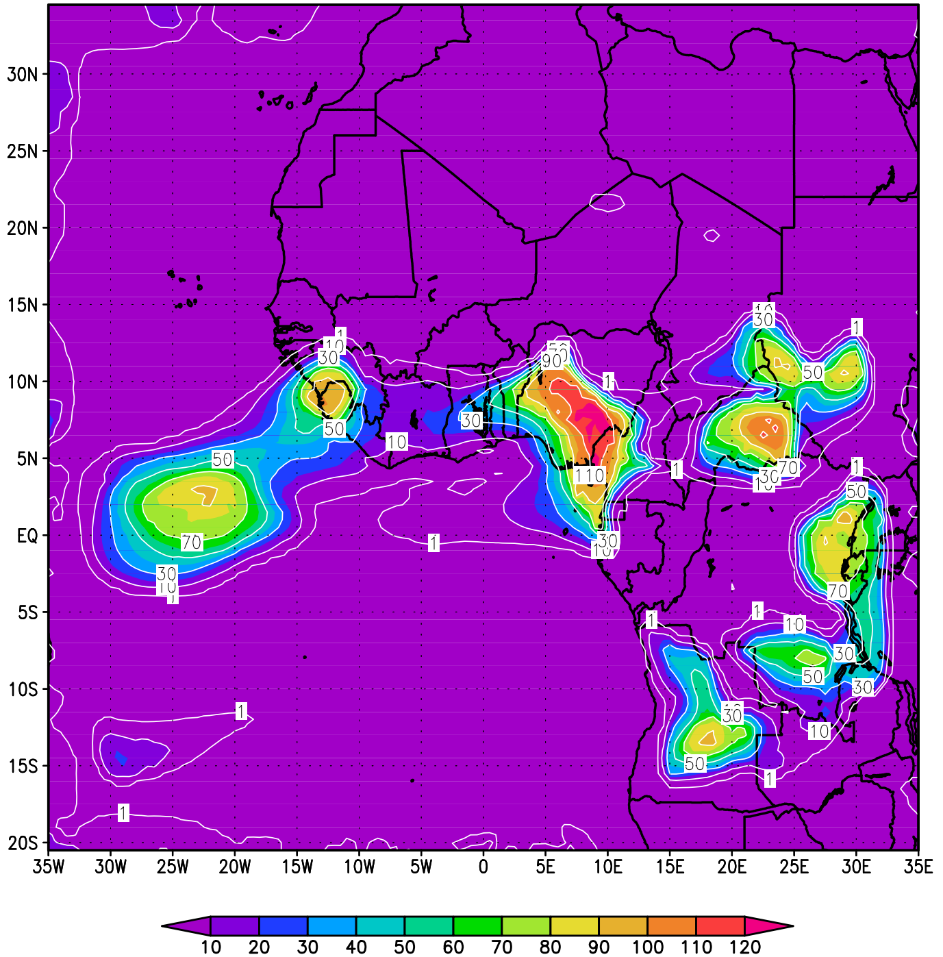
ACMAD GISS RM3 24h rainfall; valid T+72H; from 00Z on Wed Jun 8 2016
