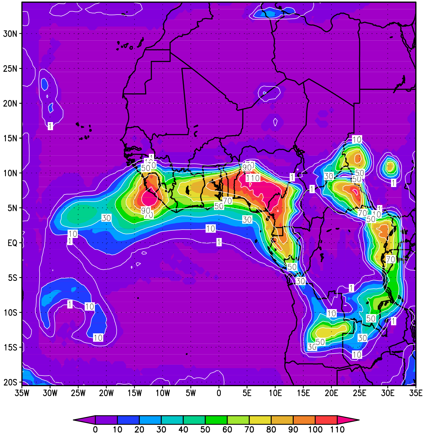
ACMAD GISS RM3 24h rainfall; valid T+72H; from 00Z on Sat Jun 11 2016
