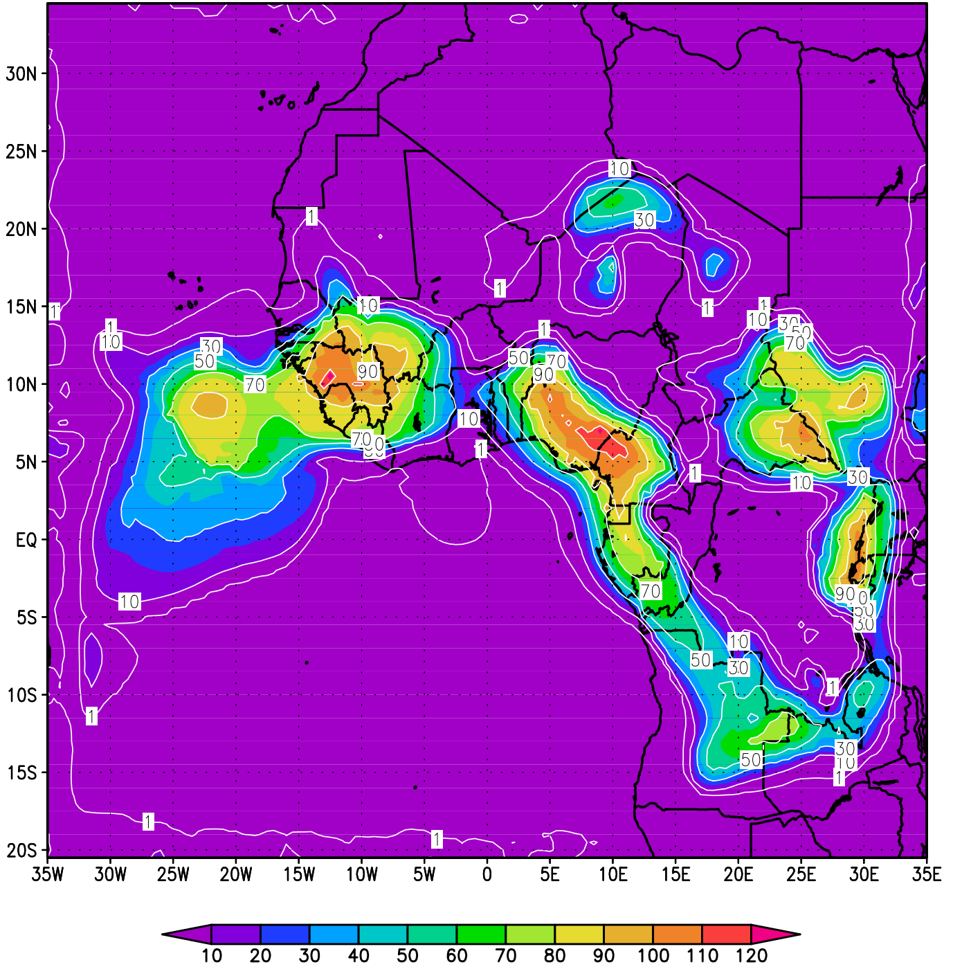
ACMAD GISS RM3 24h rainfall; valid T+72H; from 12Z on Thu Jul 21 2016
