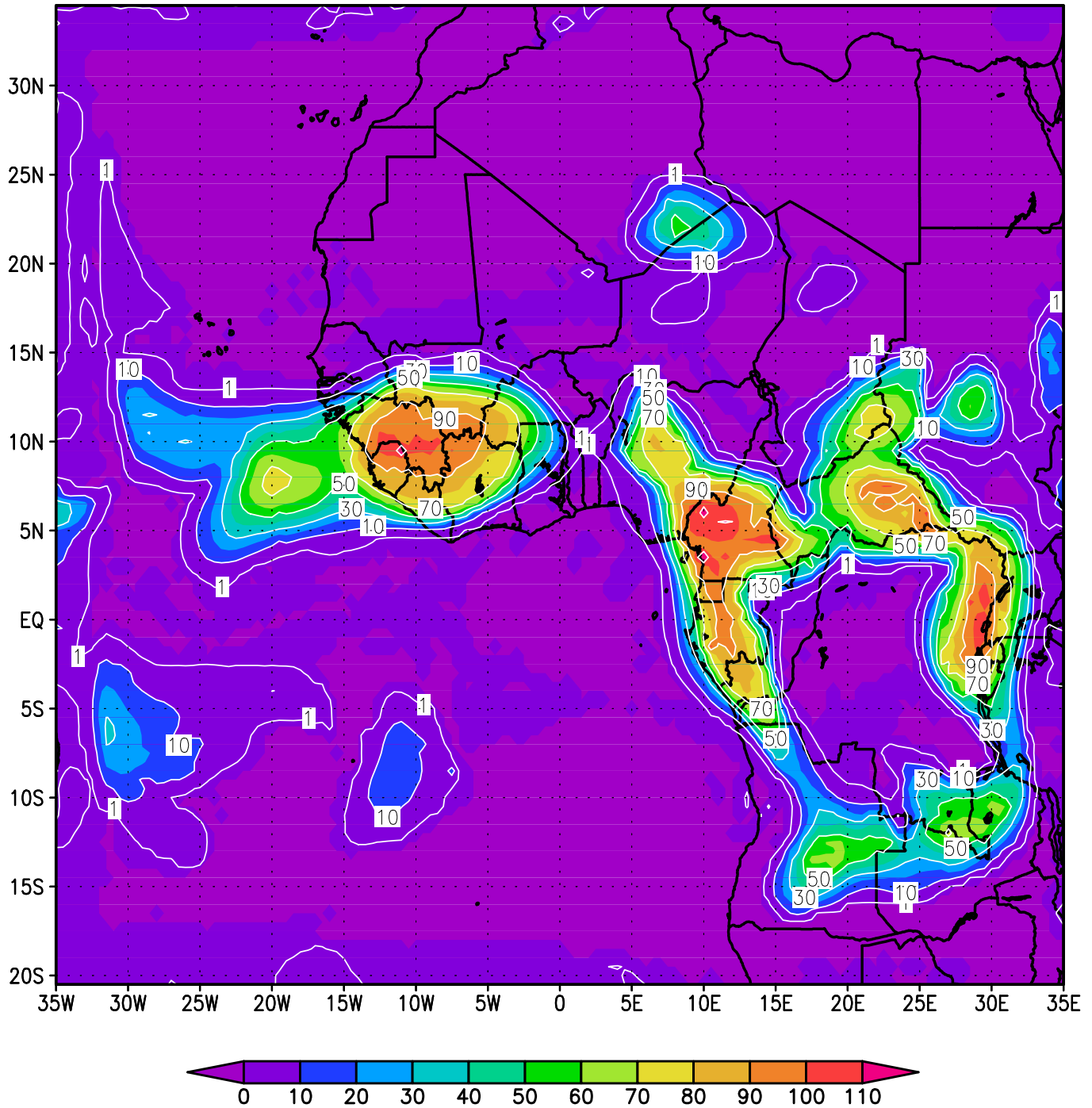
ACMAD GISS RM3 24h rainfall; valid T+48H; from 00Z on Thu Jul 21 2016
