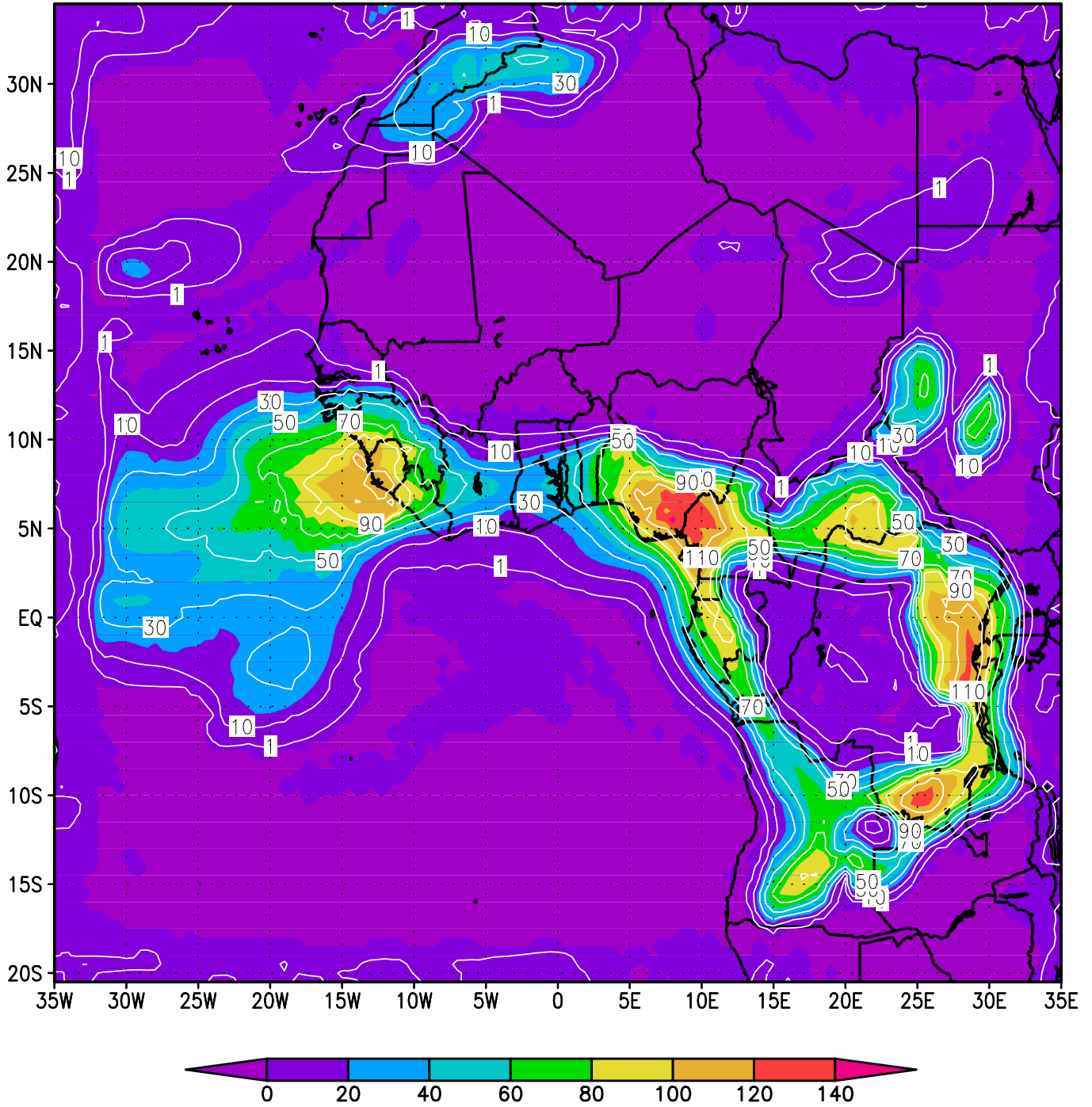
ACMAD GISS RM3 24h rainfall; valid T+72H; from 00Z on Fri Oct 23 2015
