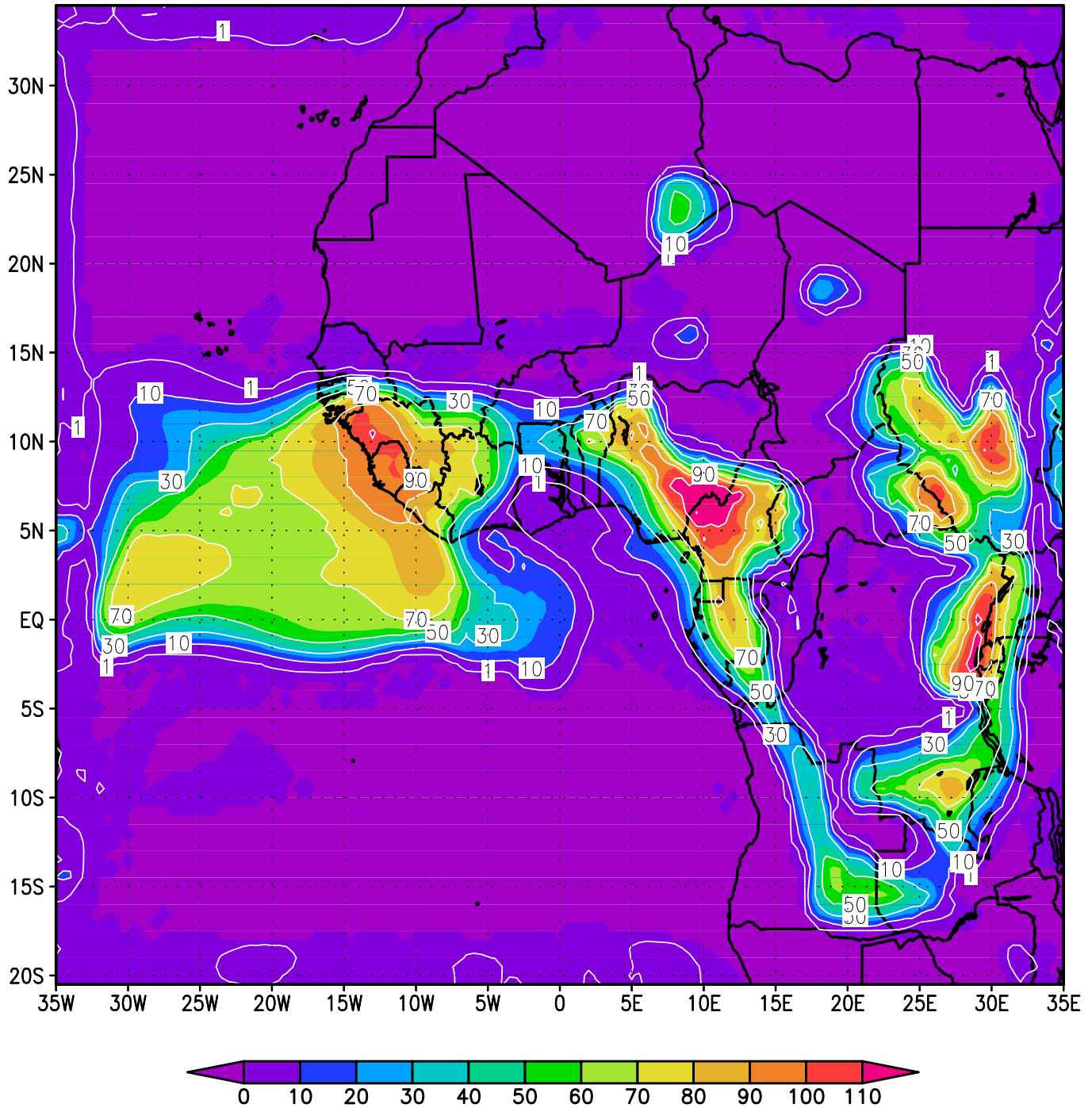
ACMAD GISS RM3 24h rainfall; valid T+72H; from 00Z on Tue Jul 26 2016
